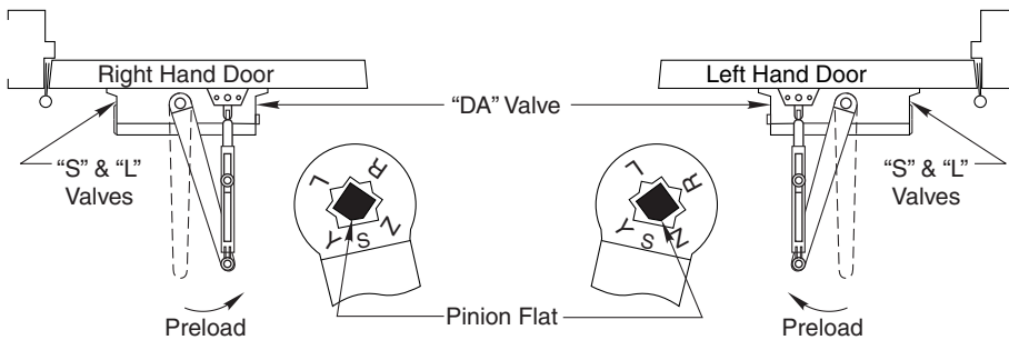
Regular Arm 1600DA Series
