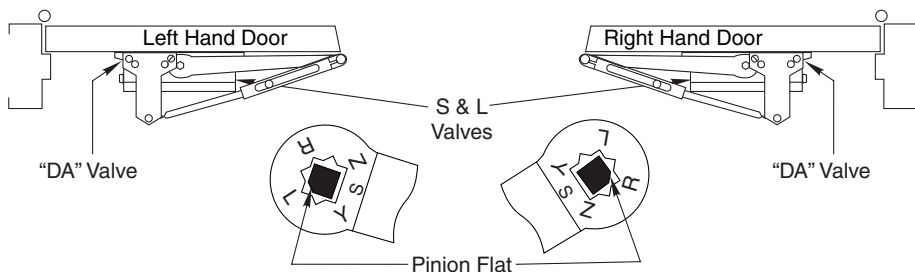
Parallel Arm P1600DA Series CLP-1600DA Series UNI-1600DA Series
