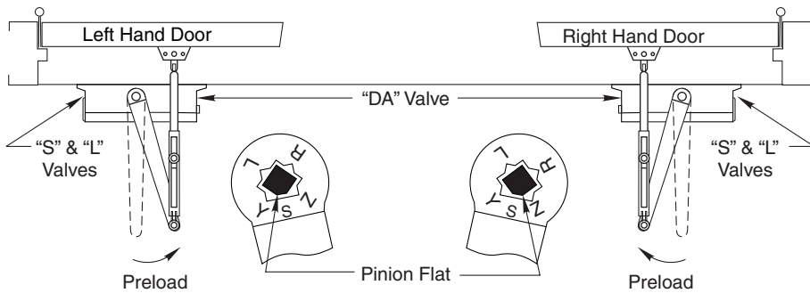
Top Jamb 1600DA Series J1600DA Series UNI-J1600DA Series
