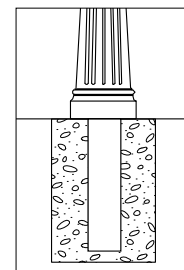
Direct In-ground Base Installation: Heavy-duty underground aluminum base extension won't rust or rot.
